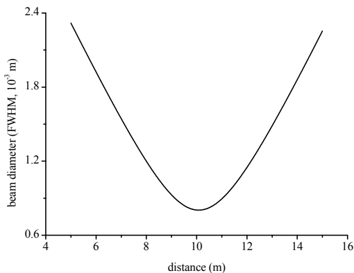
Figure 2: Seed laser beam diameter showing a focus of 0.8 mm diameter (FWHM) inside the modulator.
