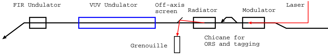
Figure 1: Schematics of the Optical Replica Synthesizer.
